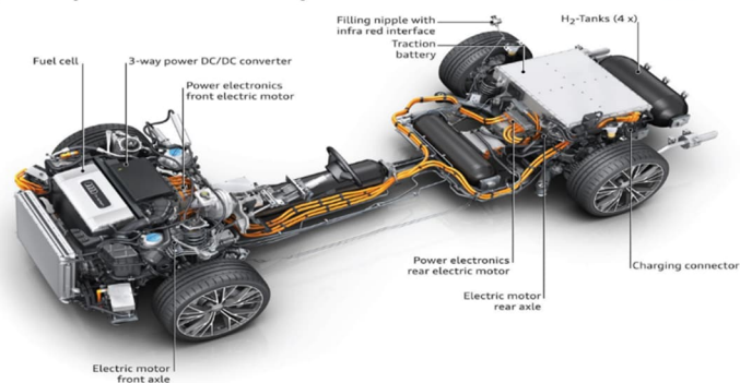
Audi A7 Sportback h-tron quattro Drivetrain 1.1/14
